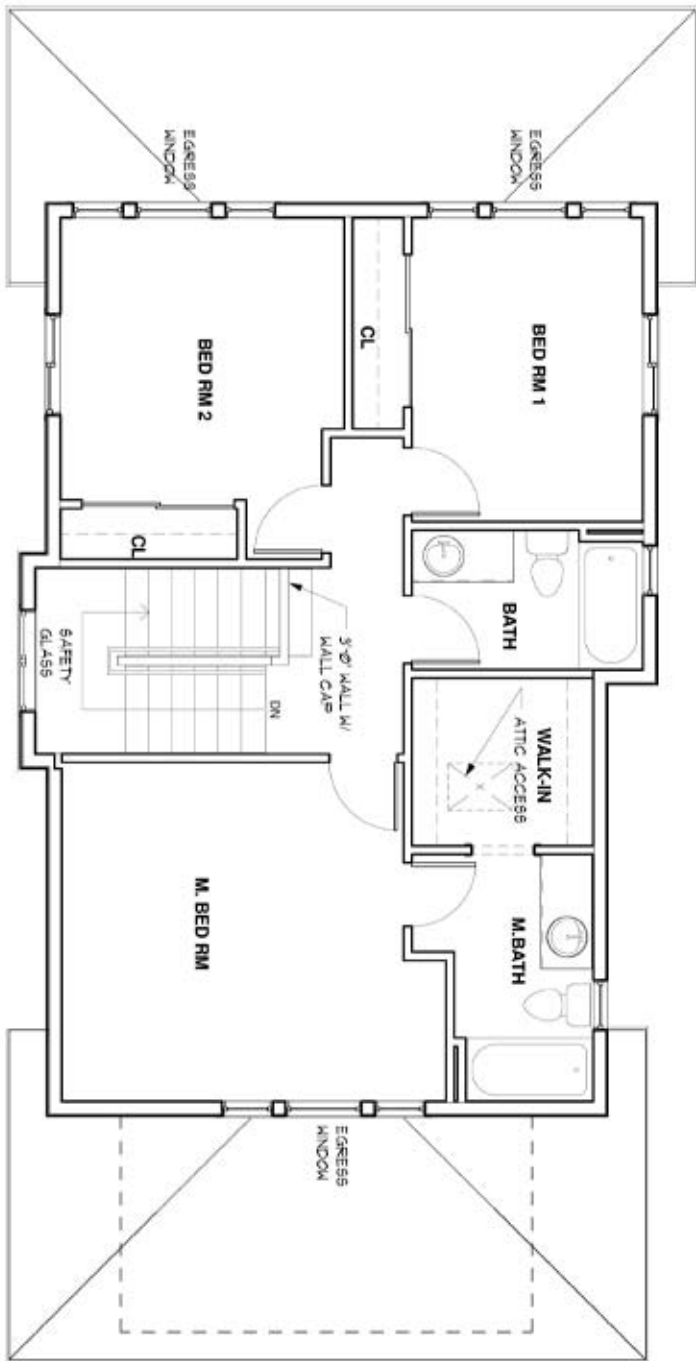
UPPER FLOOR PLAN 766 SF.
