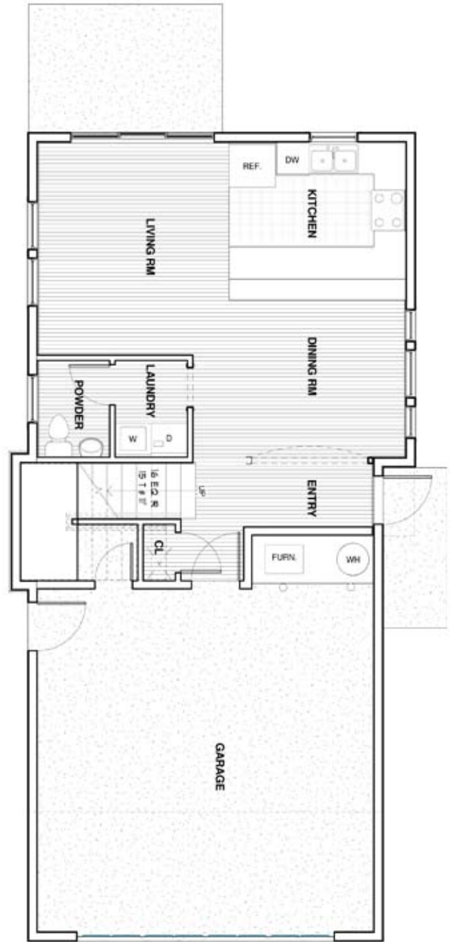
MAIN FLOOR PLAN 630 SF. Garage - 512 sf
